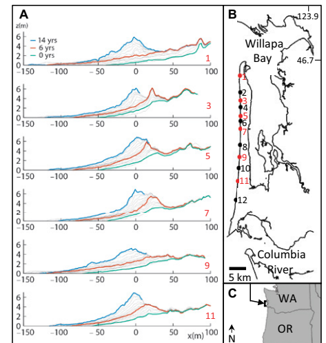
Figure 1. Representative selection of measured profiles for locations along Long Beach Peninsula, Washington State, USA. Along-shore position is given by numbers in bottom right corner of each panel, corresponding to red numbers on map. Green profiles were collected in A.D. 1998. Red profiles were collected 6 yr later (in 2004), and blue profiles were collected 14 yr later (in 2012). Elevation is relative to shoreline position (3 m contour, North American Vertical Datum of 1988). WA—Washington; OR—Oregon.
